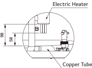
DETAILA SCALE 1 : 5
